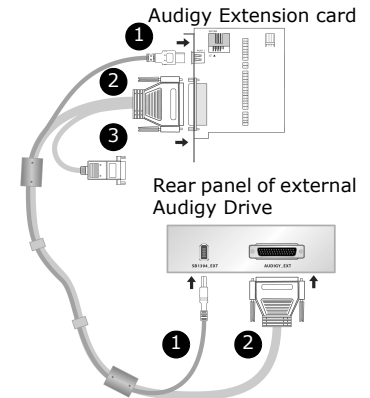
Figure 2-6: Connecting the cables to the external Audigy Drive
